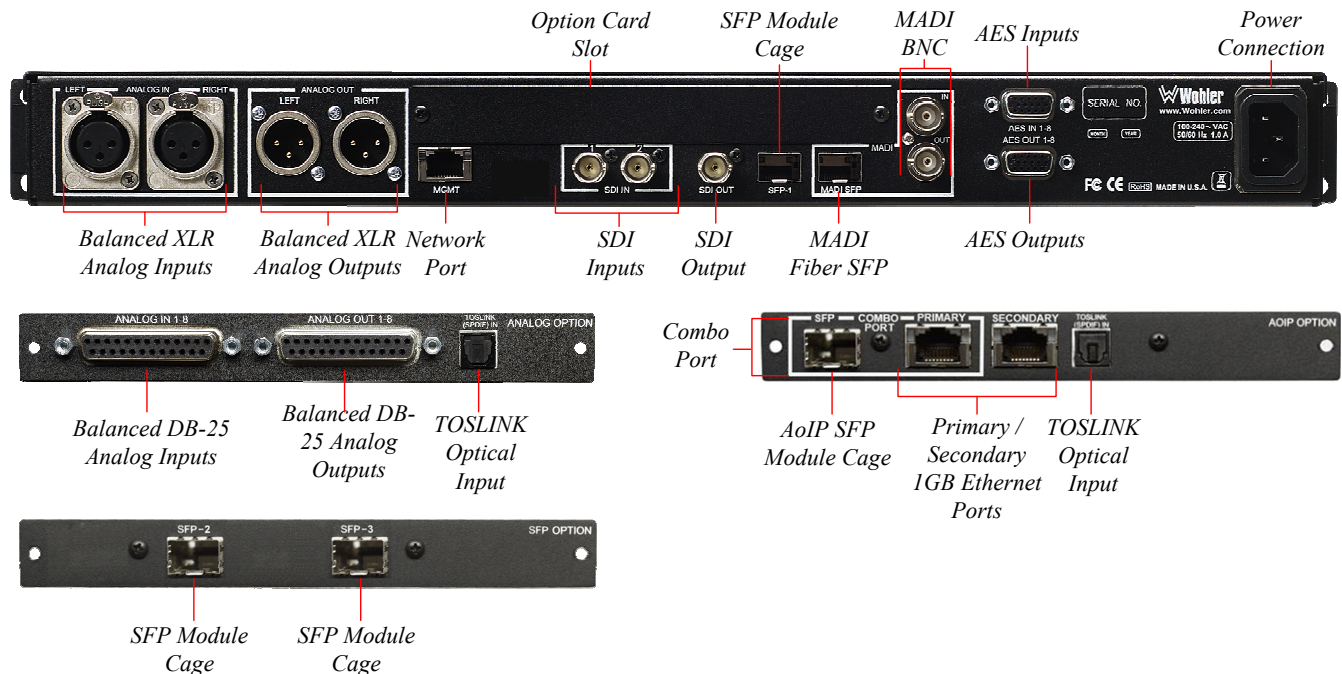
Figure 2-2: iVAM1-1 Rear Panel and Option Cards
