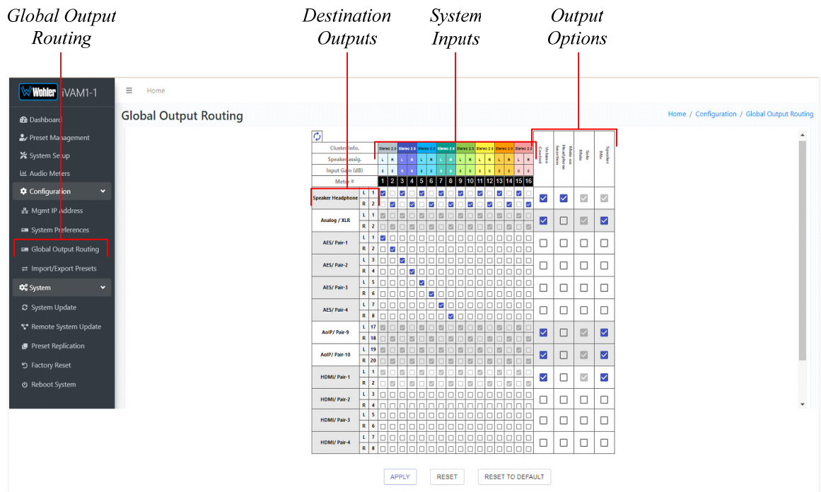
Figure 4-14: Global Output Routing Option
