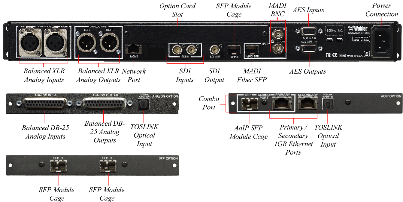
Figure 2-2: iAM1-8 Rear Panel & Option Cards
