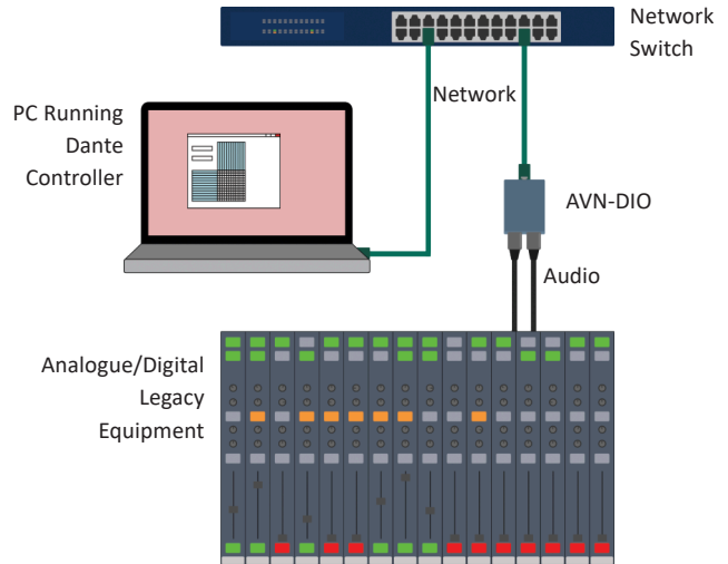
Fig 9: Typical AVN-DIO setup
