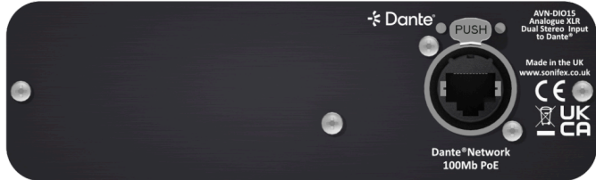
Fig 1: AVN-DIO15 Front Panel
