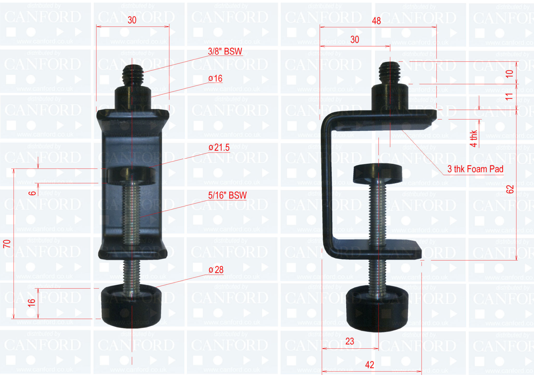
53-237 K&M 23700 G-CLAMP Clamping range 45mm, black
