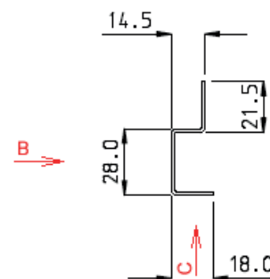
End Profile
