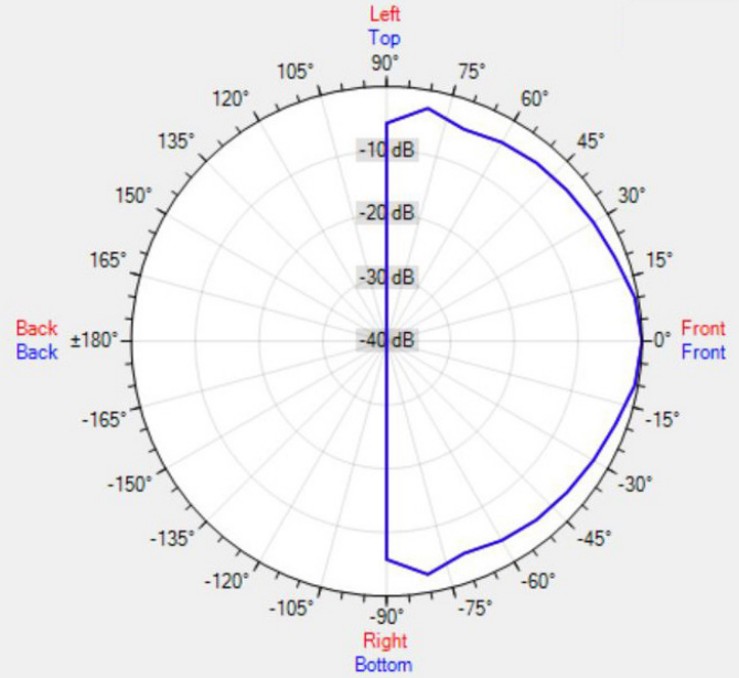
Data Shown: CMS15T (Apart Audio) Display Parameters: Frequency: 2000Hz (1/24th Octave)
