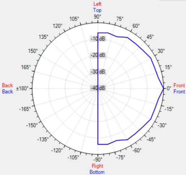
Data Shown: CMS15T (Apart Audio) Display Parameters: Frequency: 4000Hz (1/24th Octave)
