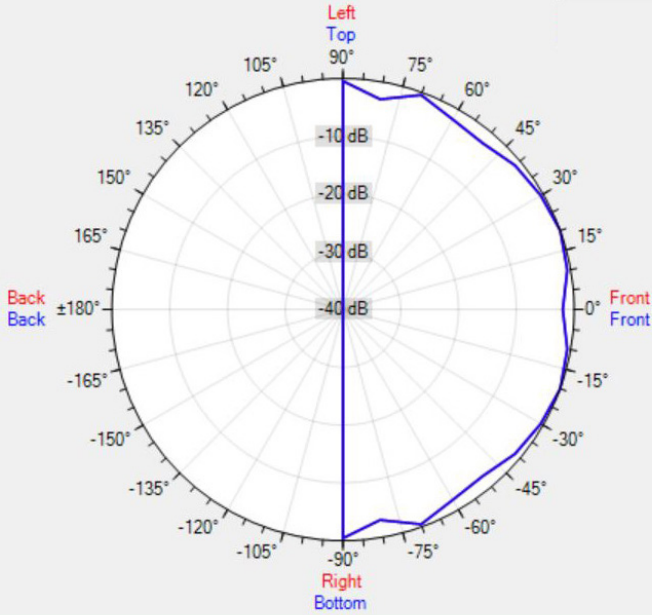
Data Shown: CMS15T (Apart Audio) Display Parameters: Frequency: 1000Hz (1/24th Octave)
