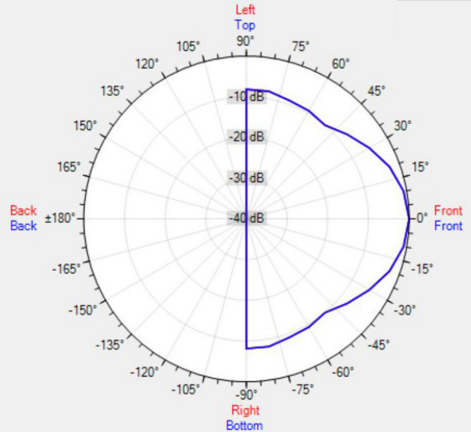
Data Shown: CMS15T (Apart Audio) Display Parameters: Frequency: 8000Hz (1/24th Octave)
